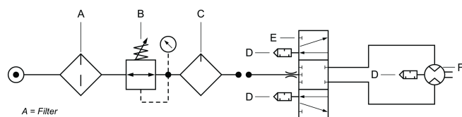
A = Filter B = Pressure regulator C = Oil fog lubricator D = Silencer E = 5/3 valve F = Motor
