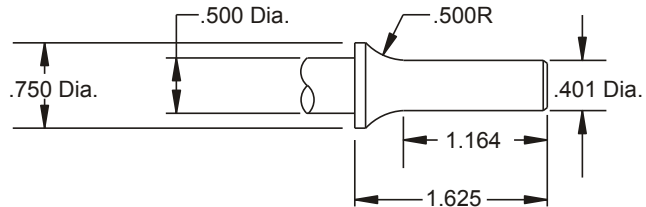
CHISEL SHANK DIMENSIONS
