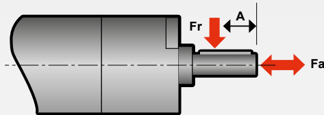
CYLINDRIC SHAFT
